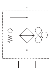
2000KBV & HPV AC Motor Series Hydraulic circuit
